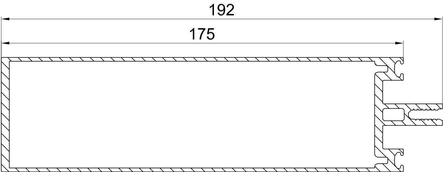
M70034 Ix=507cm 4
