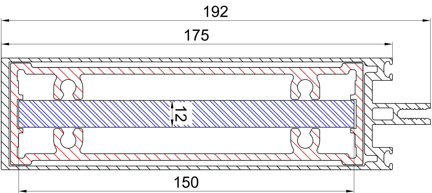
M70034+M70118+steel insert 150X12 Ix, average=2416cm 4
